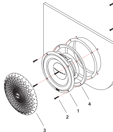
Rear Mounting
