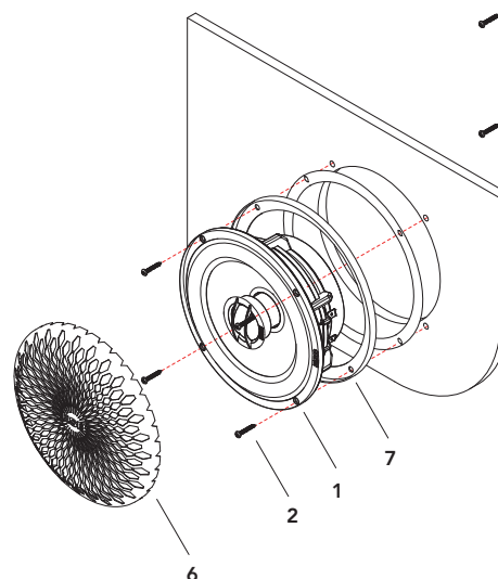
Mounting with Grille
